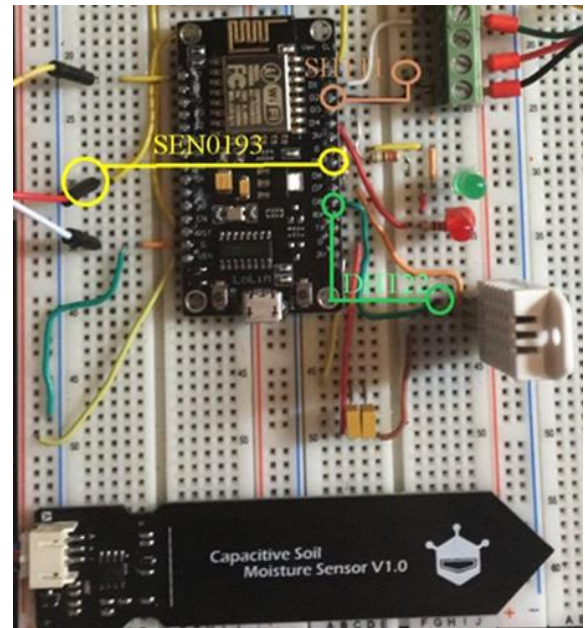
Fig. 12. View of realized sensor node with highlighted the GPIOs, set as output, used for power supplying the sensors.
