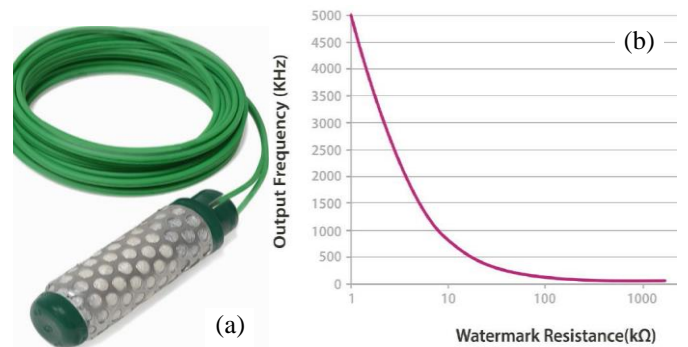
Fig. 4. View of the watermark soil moisture sensor (a) and output frequency of the Watermark sensor circuit with respect to the resistance of the sensor (b).
