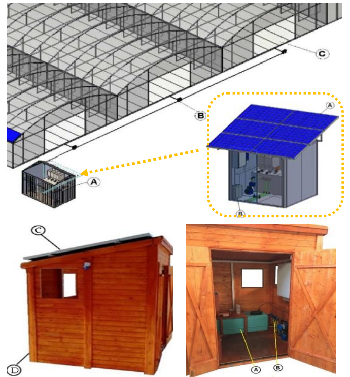
Fig. 8. Whole designed fertigation system for greenhouses and in zoomed area the solar powered wooden cottage with inside the fertigation system and batteries for energy storage (B); real images of wooden cottage (D) with inside electronic and mechanical sections with mixing tank (A), solenoid valves for selecting the land's sectors to be irrigated (B) and solar panels (C).
