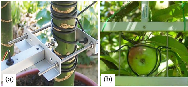
Fig. 6. Electronic dendrometer installed on a stem (a) and a fruit (b) for detecting in real time their growing.
