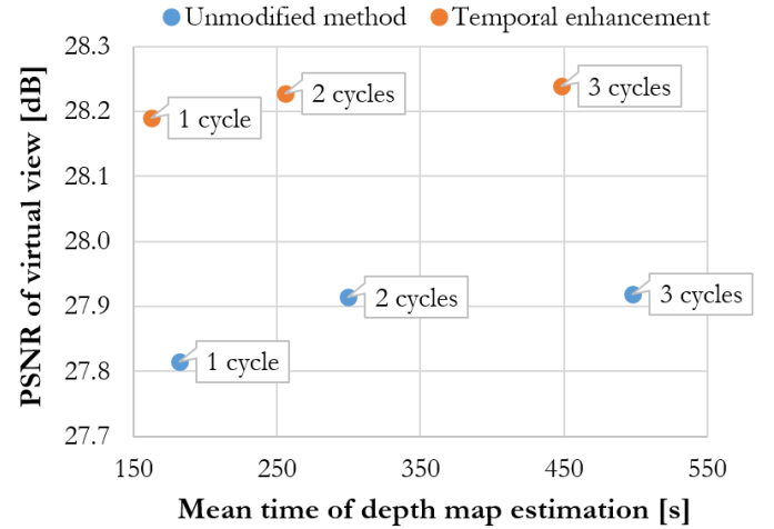
Fig. 3. Comparison of the mean quality of virtual views and the mean time of depth estimation for unmodified and proposed method.
