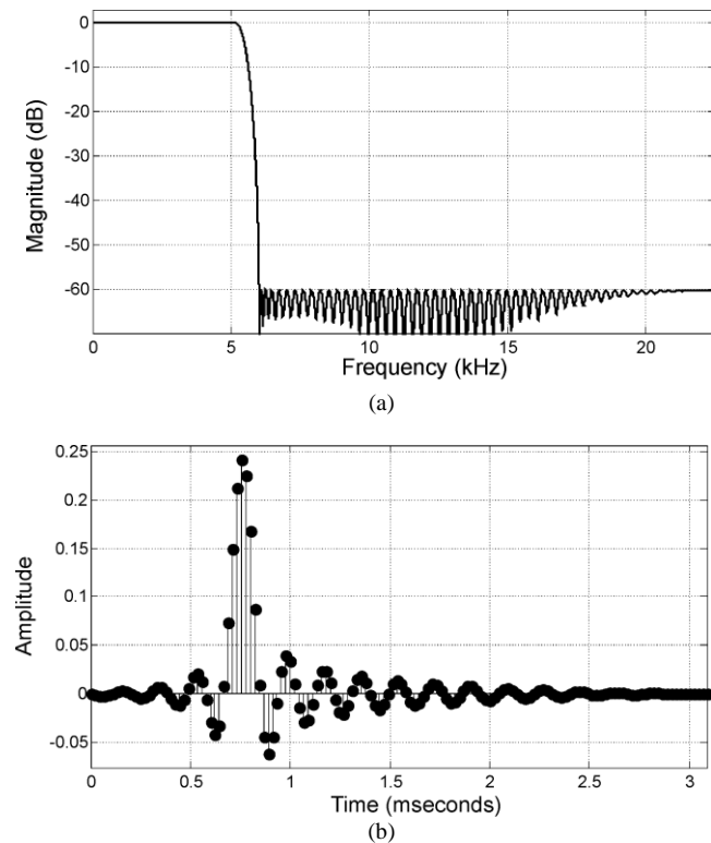
Fig. 4 Magnitude response (a) and impulse response (b) of the filter in Example 1
