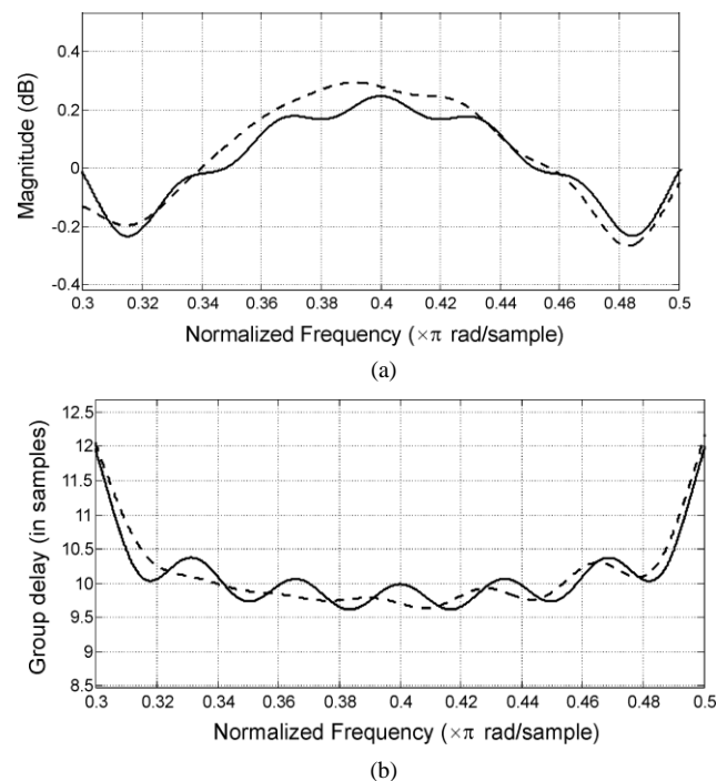
Fig. 7 Frequency responses of the filter in Example 2, (a) magnitude response in passband and (b) group delay response obtained after first stage (solid line) and second stage (dashed line) of proposed algorithm
