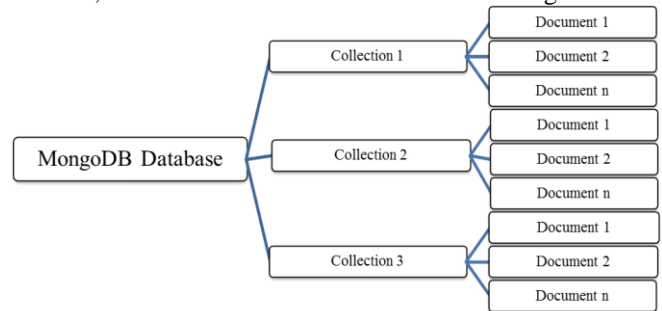
Fig. 2. MongoDB structure.
