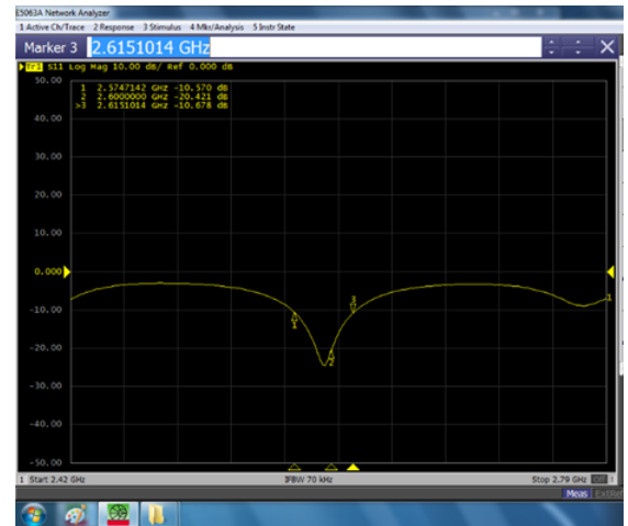
Fig. 24. Return loss measurement results for a 1x5 microstrip antenna with a parasitic patch and proximity coupling
