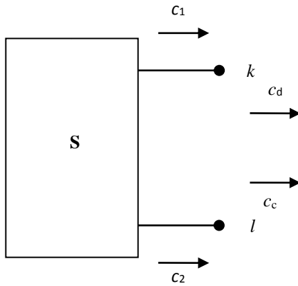
Fig. 2. Differential signal source with noise waves at its ports
