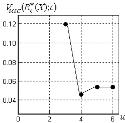
Fig. 3. Plot of the measure of separation and compactness for Sneath and Sokal's data set.
