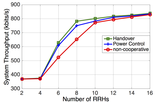
Fig. 7. Average Throughput: Handover Versus Power Control
