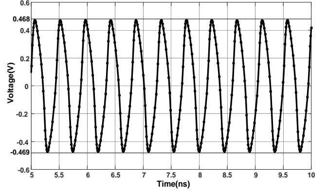
Fig. 9(a). Differential output voltage vs time for Weng-Kuo cascode active inductor based VCO.
