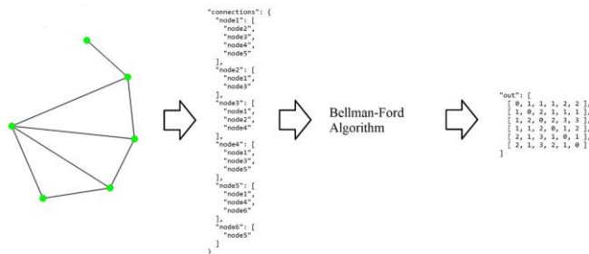
Fig. 3. Connections map and distances matrix descriptions for the presented cluster in JSON format, nodes in the cluster are encountered counterclockwise
