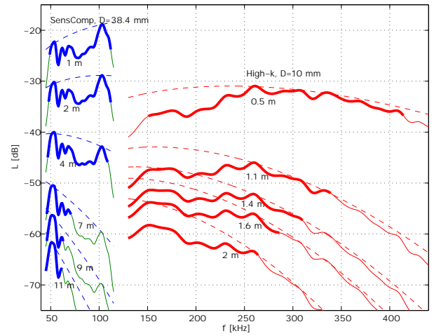
Fig. 1. Frequency response of the channel with different transducers
