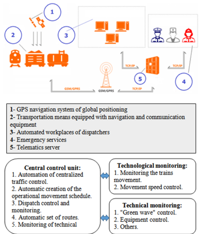
Fig. 1. Scheme of information exchange of the automated dispatch control system and HSRWT movement coordination system
