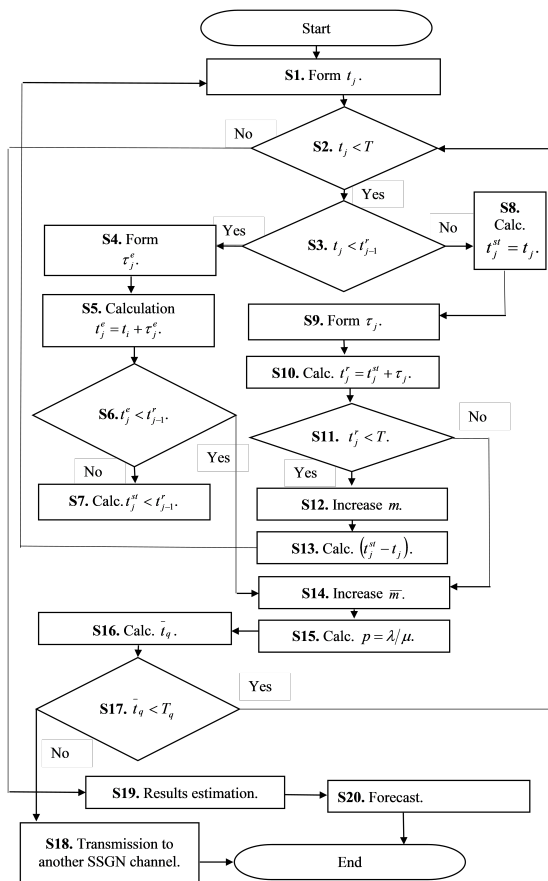
Fig. 5. The block diagram of the algorithm for the simulation of the GPRS channels operation as a part of the ADCS data transmission subsystem
