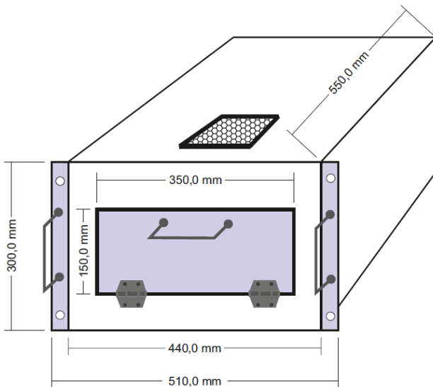
Fig. 5. Dimensions of the enclosure.
