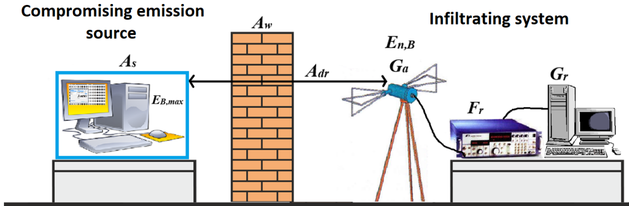
Fig. 1. The energy budget of the link between the secured IT equipment and the potential infiltrating system.
