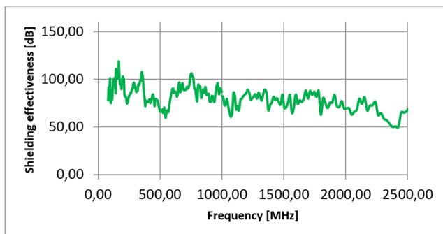
Fig. 7. Resulting A_s of the shielding enclosure.
