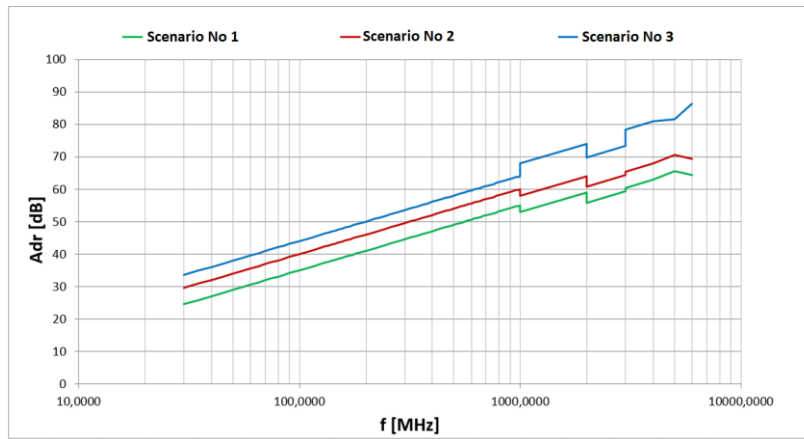
Fig. 3. Attenuation A_{dr} introduced by signal propagation path for particular scenarios of IT equipment location in relation to the location of the infiltrating system.
