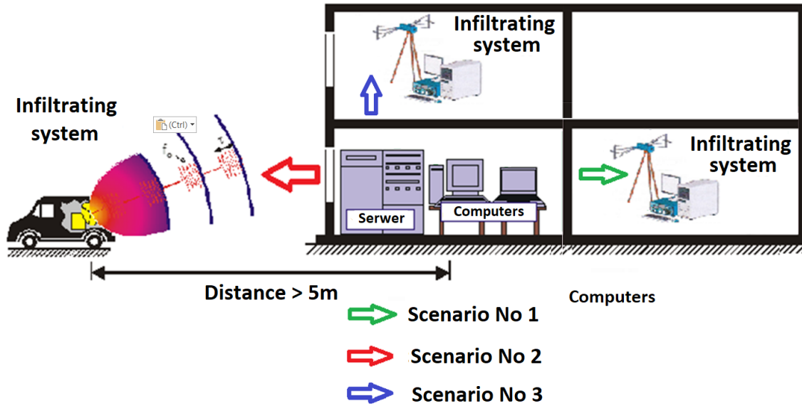
Fig. 2. Graphical representation of IT equipment and infiltrating system location scenarios.
