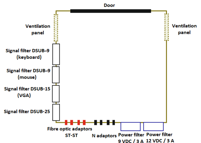
Fig. 4. Block diagram of the enclosure.
