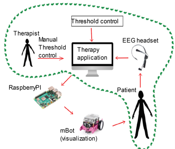
Fig. 3. Block diagram of the system
