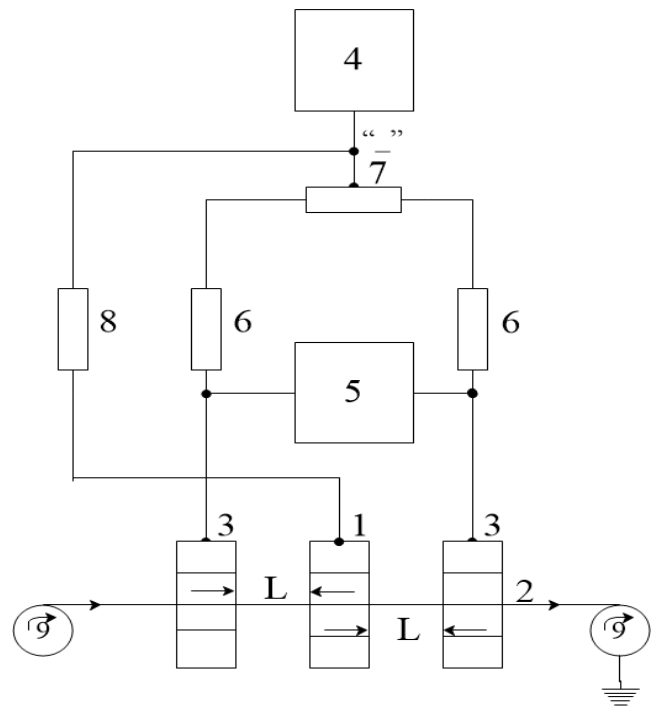
Fig.4. Functional diagram of a device for measuring the speed of a microwire drawing during its manufacture
