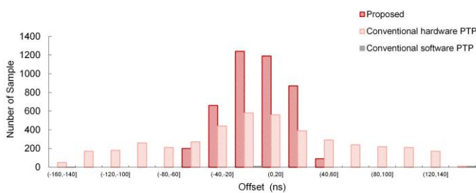
Fig. 14. The time offset histogram
