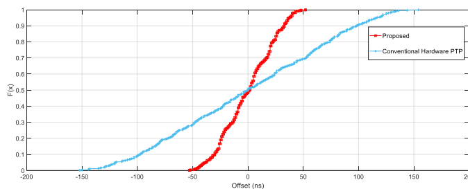
Fig. 12. The Cumulative Distribution Function of the offset
