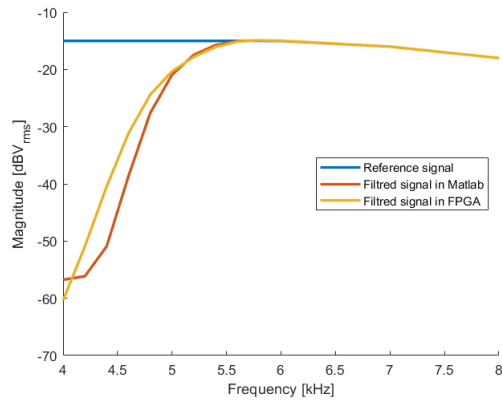
(c) Characteristic of the 5 kHz high-pass filter
