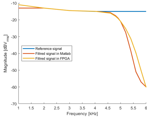
(a) Characteristic of the 5 kHz low-pass filter
