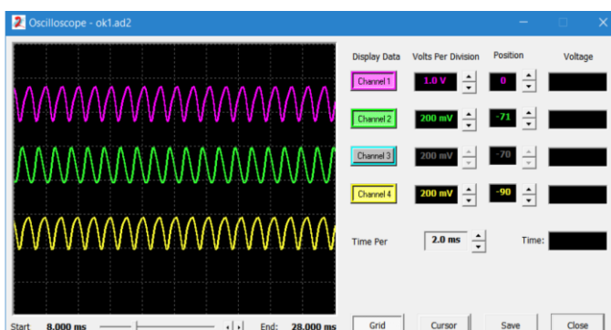
Fig. 14. Windmi Chaotic System output at a = 0.1 , b = 1
