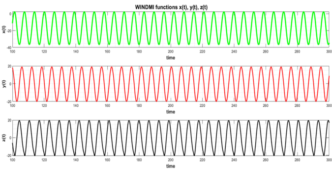
Fig. 8. Time Series at a = 0.1 and b = 1 .
