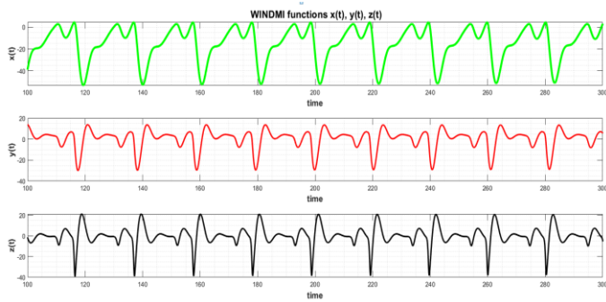
Fig.7. Time Series at a = 0.7 and b = 3.5
