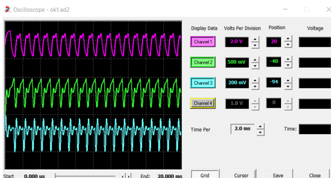
Fig. 14. Windmi Chaotic System output at a = 0.7 , b = 3.5
