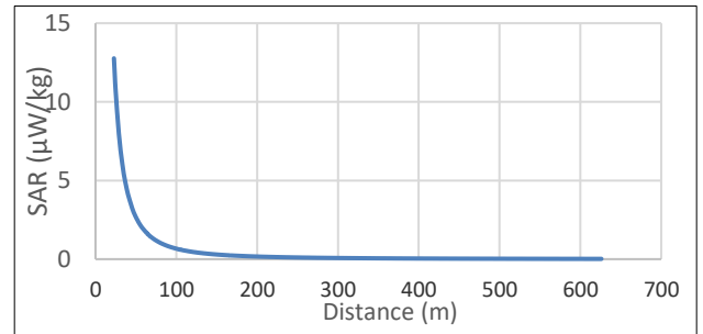
Fig.12. SAR of Alkhoud_4G Cell-34
