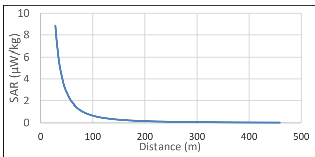
Fig.10. SAR of Alkhair_4G Cell-98
