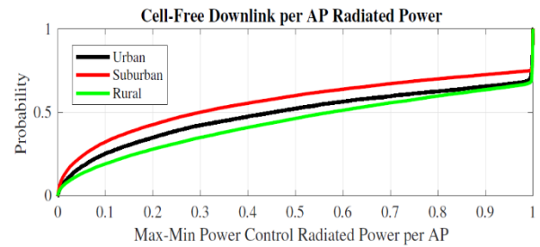
Fig. 11. Cell-free Massive MIMO with Max-Min power control strategy having transmit power normalized per AP [23]
