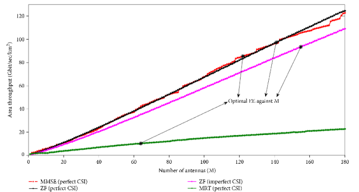
Fig. 8. Comparison of area throughput [2]
