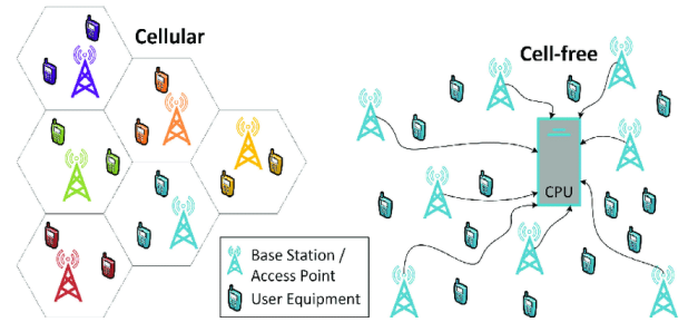
Fig. 9. Cell-free v/s cellular networks [23]
