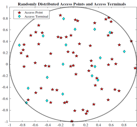
Fig. 10. Cell free Massive MIMO: M=64 AP and K=18 AT [23]
