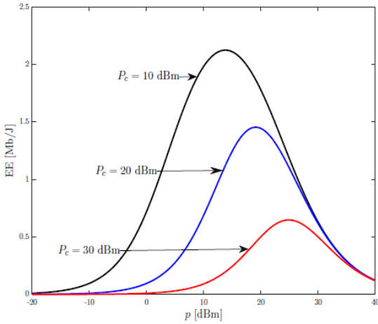
Fig. 4. Energy efficiency changes with transmit power [4]
