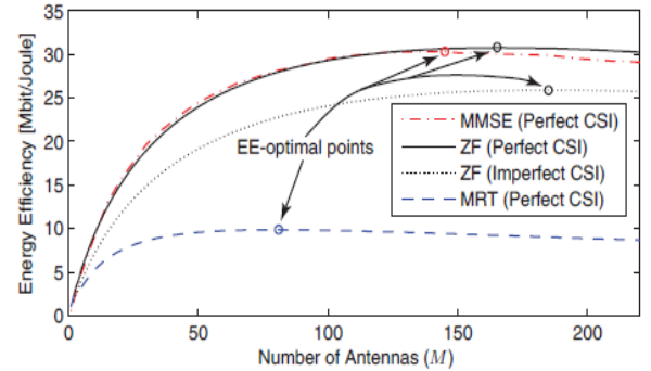
Fig. 7. Comparison of EE of different precoding schemes [2]
