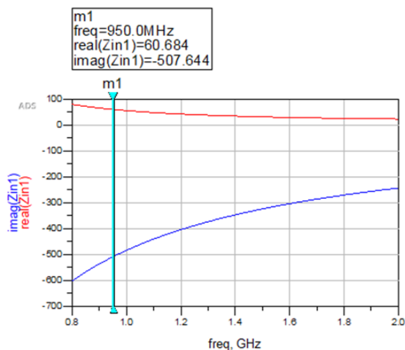
Fig. 3. Input impedance before matching with GSM 900 downlink frequency input of -10dbm source
