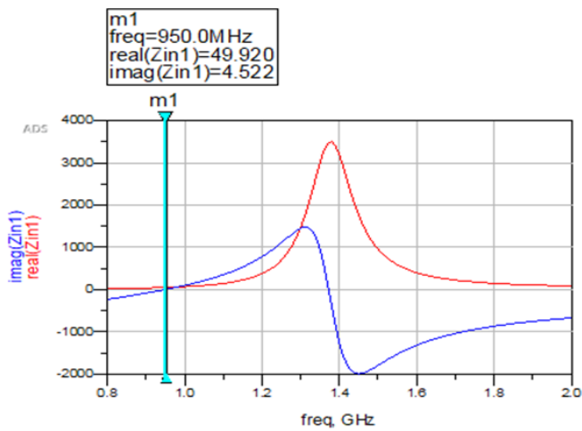
Fig. 17. Input Impedance after matching with GSM 900 downlink frequency input of -10dbm source
