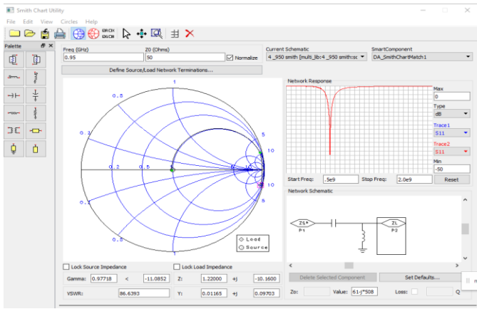
Fig. 12. Smith chart utility for impedance matching using capacitor and inductor with GSM 900 downlink frequency input of -10dbm source
