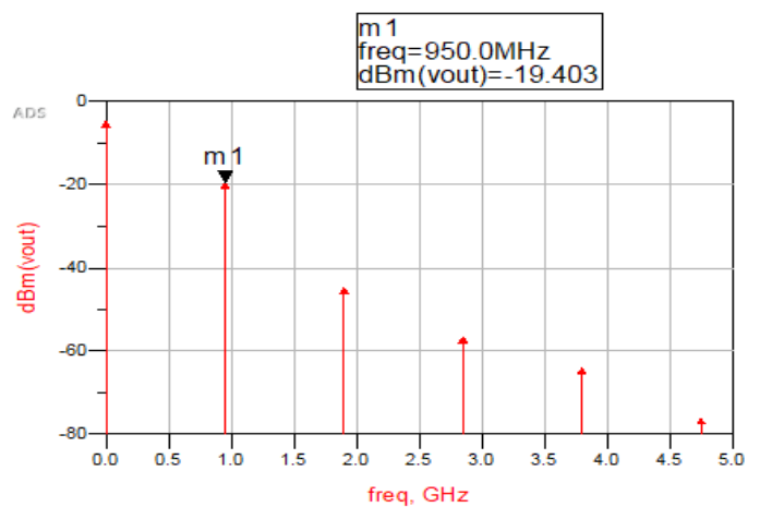
Fig. 5. Output power without matching with GSM 900 downlink frequency input of -10dbm source
