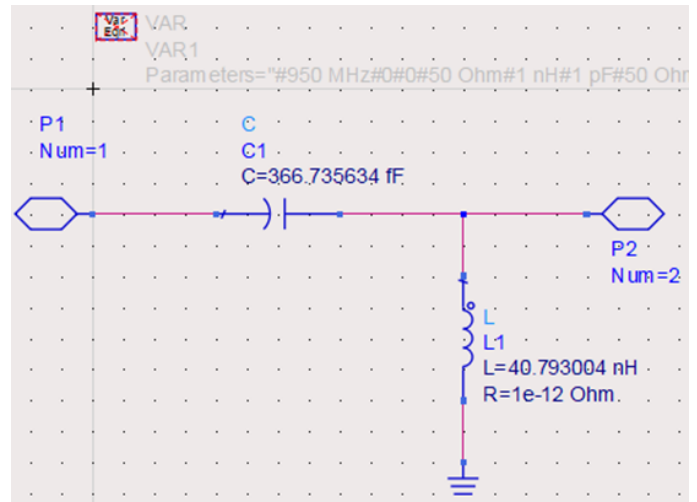
Fig. 14. Designed High Pass Impedance Matching Circuit with GSM 900 downlink frequency input of -10dbm source
