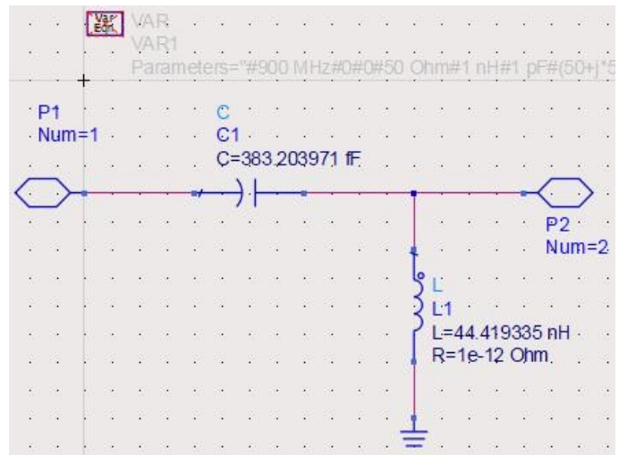
Fig. 20. Designed High Pass Impedance Matching Circuit with GSM 900 uplink frequency input of -10dbm source
