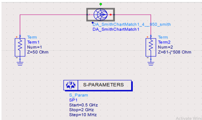
Fig. 13. Smith chart connection in ADS for impedance matching with GSM 900 downlink frequency input of -10dbm source
