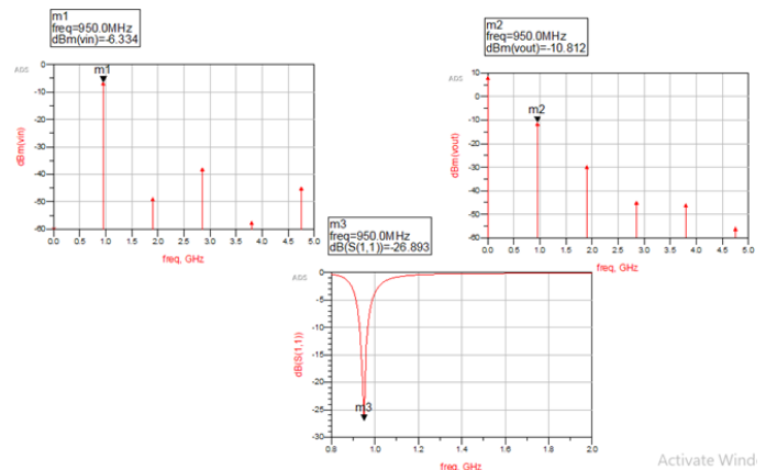
Fig. 16. After matching v_{in} (input power), v_{out} (output power), reflection coefficient S_{11} with GSM 900 downlink frequency input of -10dbm source
