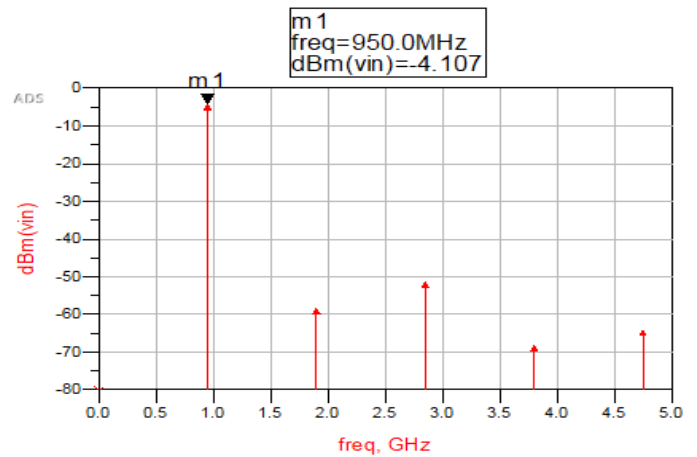
Fig. 4. input power without matching with GSM 900 downlink frequency input of -10dbm source
