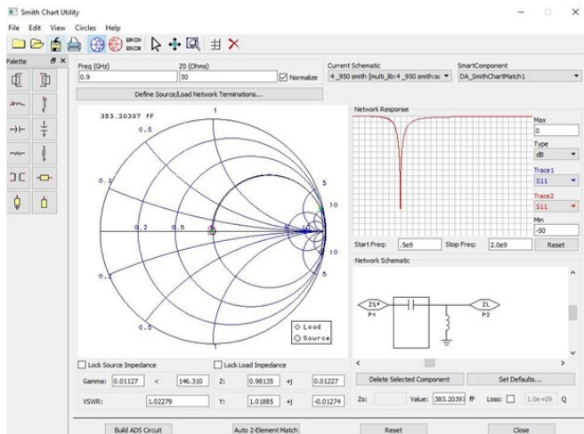
Fig. 18. Smith chart utility for impedance matching using capacitor and inductor with GSM 900 uplink frequency input of -10dbm source
