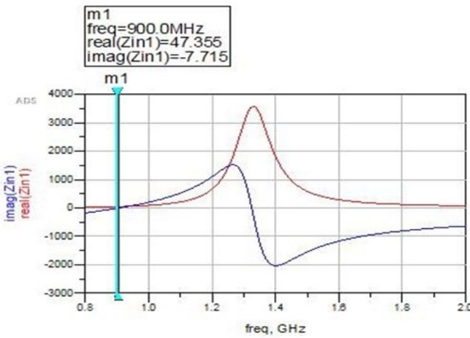
Fig. 23. Input Impedance after matching with GSM 900 uplink frequency input of -10dbm source
