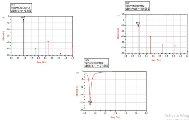
Fig. 22. After matching v_{in} (input power), v_{out} (output power), reflection coefficient S11 with GSM 900 uplink frequency input of -10dbm source
