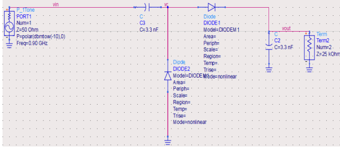
Fig. 7. A single stage Villard voltage multiplier circuit with GSM 900 uplink frequency input of -10dbm source
