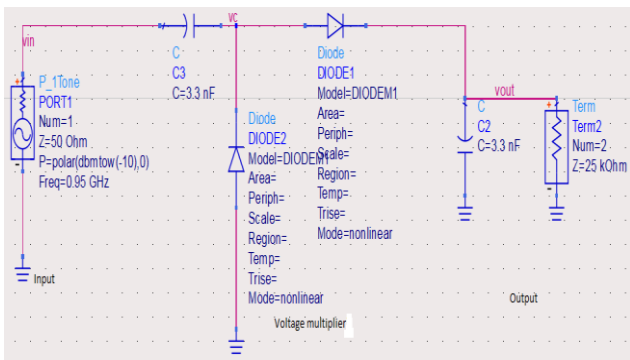
Fig. 2. A single stage Villard voltage multiplier circuit with GSM 900 downlink frequency input of -10dbm source
