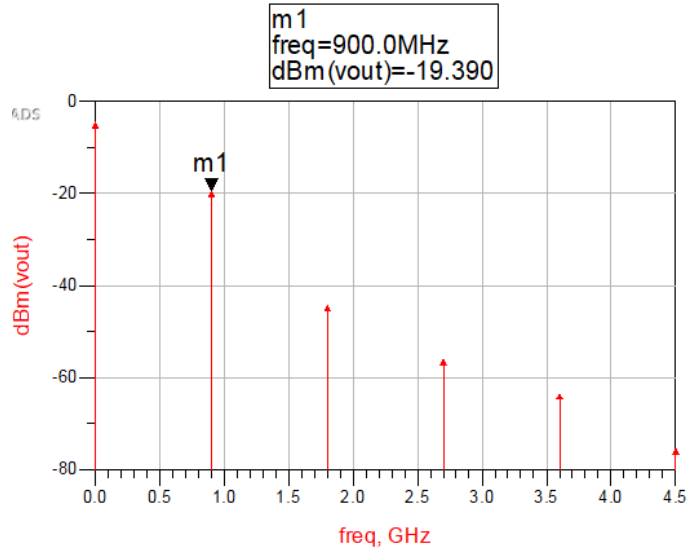
Fig. 10. Output power without matching with GSM 900 uplink frequency input of -10dbm source
