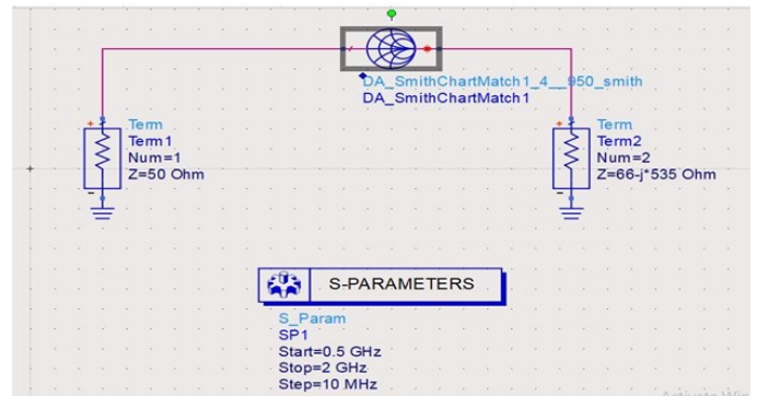
Fig. 19. Smith chart connection in ADS for impedance matching with GSM 900 uplink frequency input of -10dbm source
