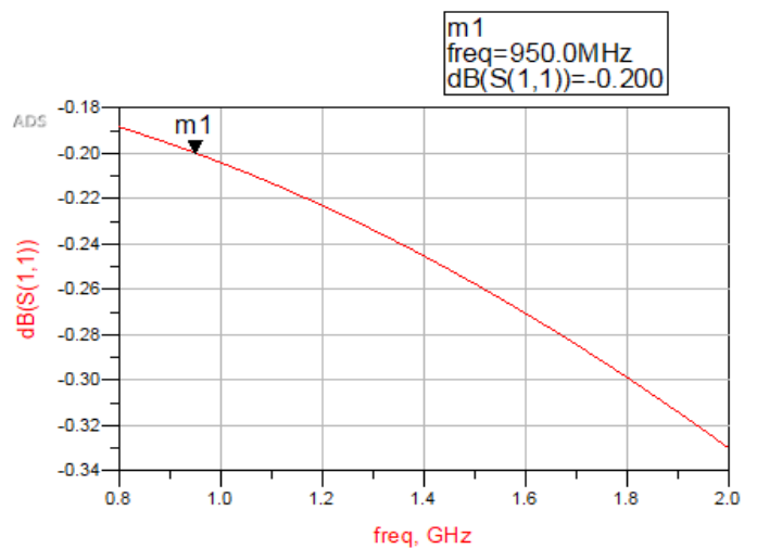
Fig. 6. reflection coefficient ( S_{11} ) before matching with GSM 900 downlink frequency input of -10dbm source
