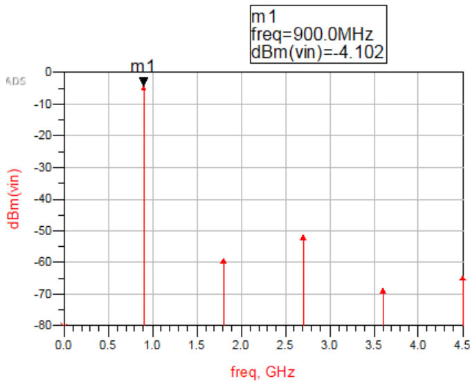
Fig. 9. input power without matching with GSM 900 uplink frequency input of -10dbm source
