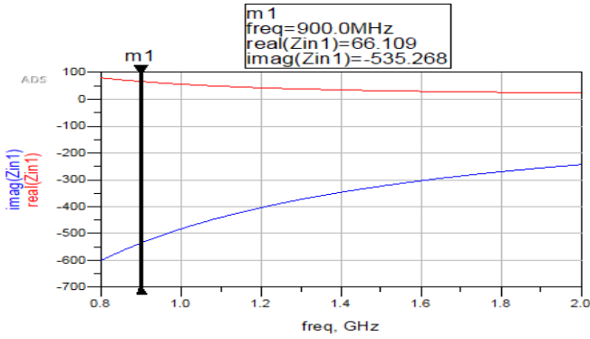
Fig. 8. Input impedance before matching with GSM 900 uplink frequency input of -10dbm source
