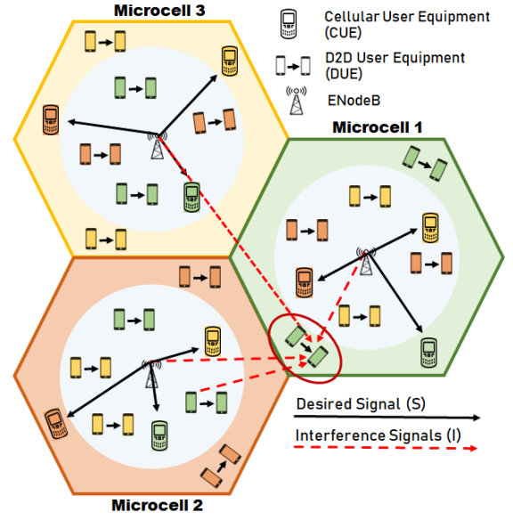
Fig. 4. Three microcells of cellular network with the proposed FFR scheme for observed DUE receiver at cell edge.
