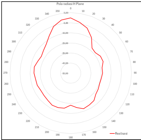
Fig. 11. H-Plane Radiation Pattern of the Realized Microstrip Array Antenna
