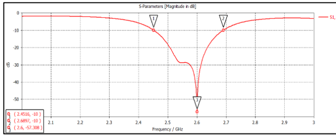
Fig. 2. S11 Value of the 4-Element Microstrip Array Antenna
