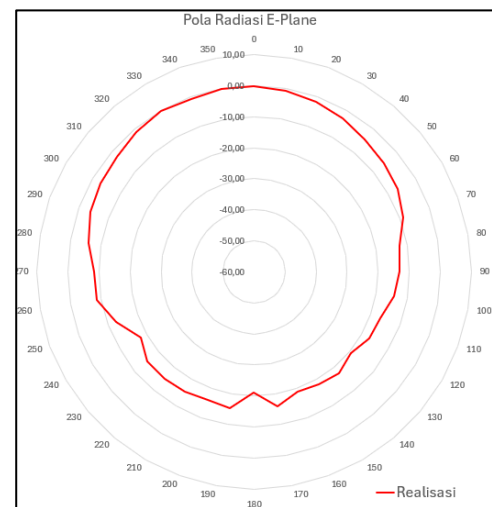
Fig. 9. E-Plane Radiation Pattern of the Realized Microstrip Array Antenna
