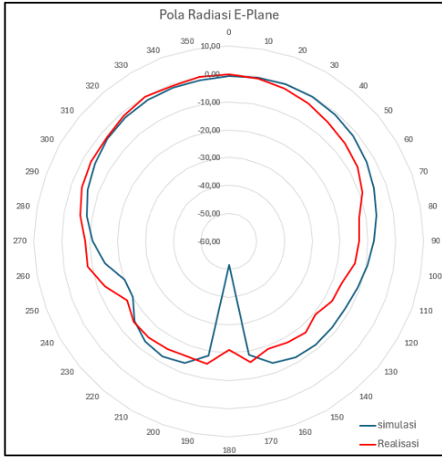
Fig. 10. Comparison of E-Plane Radiation Patterns Between Simulated and Realized Antennas
