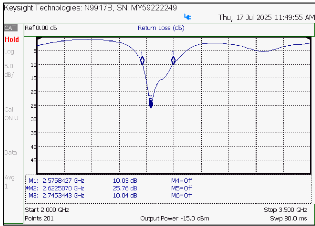
Fig. 7. S11 Value of the Fabricated 4-Element Microstrip Array Antenna
