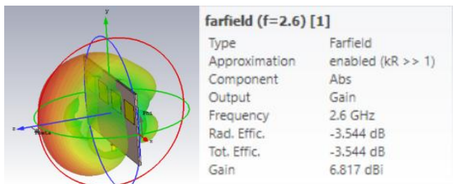
Fig. 3. Gain Value of the 4-Element Microstrip Array Antenna
