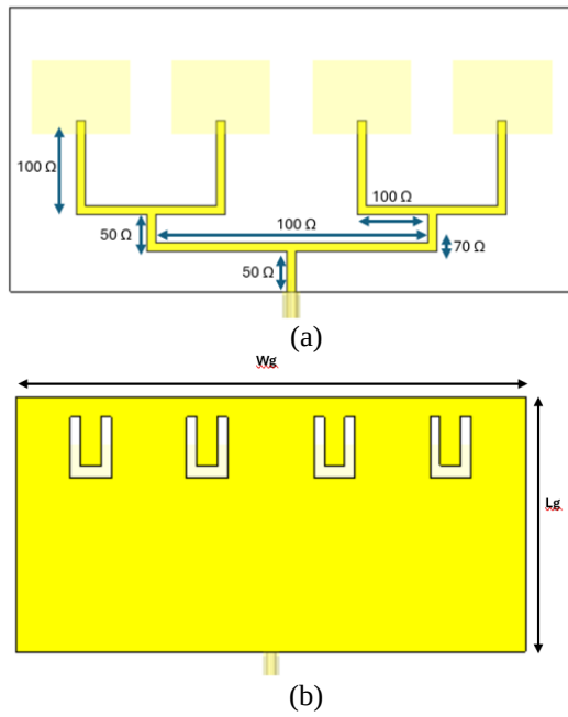
Fig. 1. (a) Front view of the 4-element microstrip array antenna design (b) Rear view of the 4-element microstrip array antenna design
