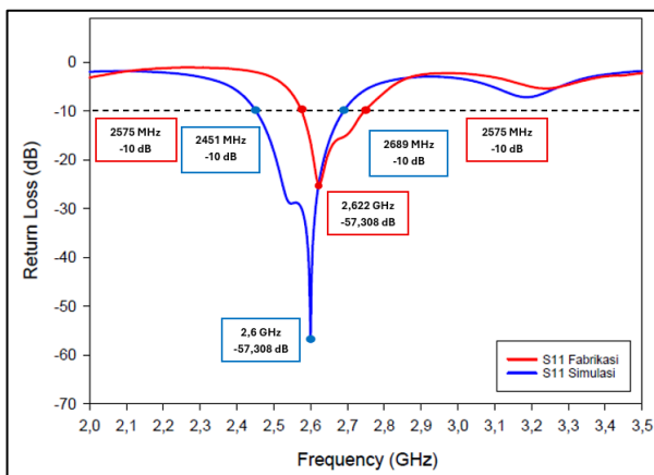
Fig. 8. Comparison Graph of Simulation and Fabrication Results of the 4-Element Microstrip Array Antenna
