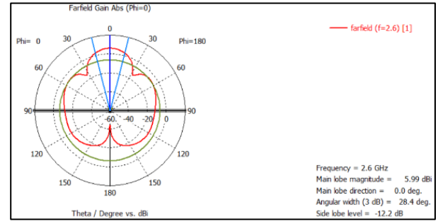
Fig. 5. H-Plane Phi = 0 Radiation Pattern of the 4-Element Microstrip Array Antenna
