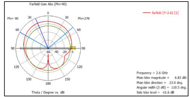
Fig. 4. E-Plane Phi = 90 Radiation Pattern of the 4-Element Microstrip Array Antenna
