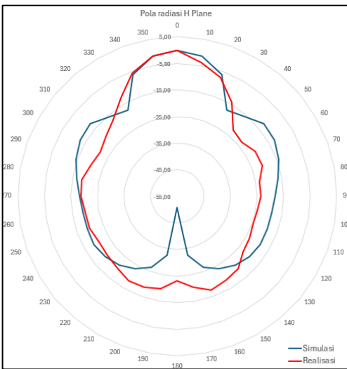
Fig. 12. Comparison of H-Plane Radiation Patterns Between Simulated and Realized Antennas
