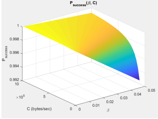
Fig. 3. Combined impact of channel degradation \beta and throughput C on the probability of successful recovery P_{success}
