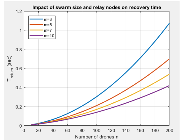
Fig 5. The impact of drone swarm size and number of relay nodes on the drone recovery time
