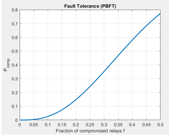
Fig. 4. Probability of system compromise P_{comp} versus fraction of malicious relay nodes f in a PBFT consensus model
