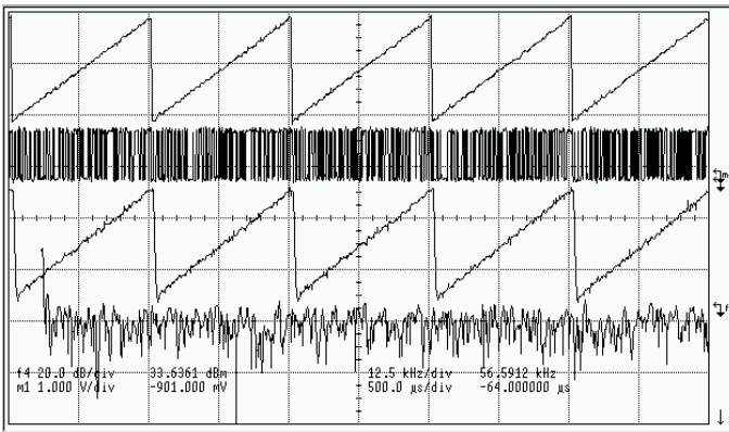
Fig. 7. Linear ramp input and output waveforms of the standard third-order \Sigma\Delta ADC.
